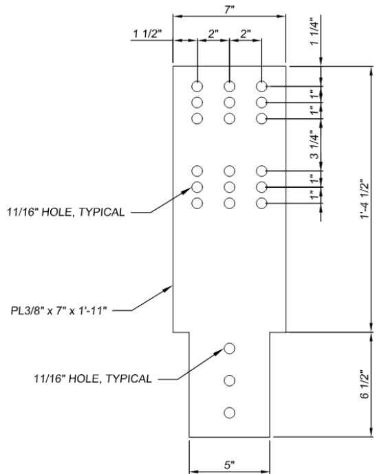
I-BEAM ADAPTOR PLATE 3/8" Thick Steel Plate Finish: Hot-Dip Galvanized (HDG)
