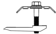
MID CLAMP ASSEMBLY
