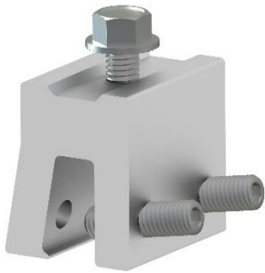
1" SEAM CLAMP STANDARD K50200-001
